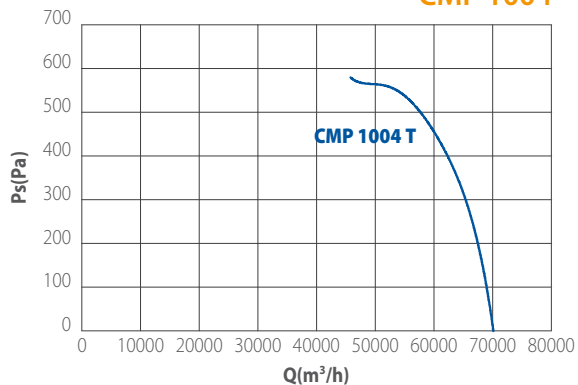
CMP 1004
