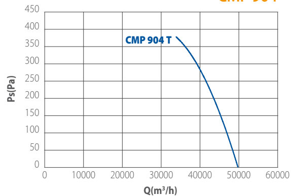
CMP 904
