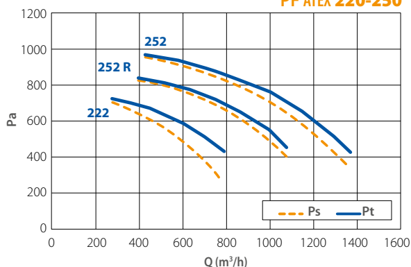
PF ATEX 220-250
