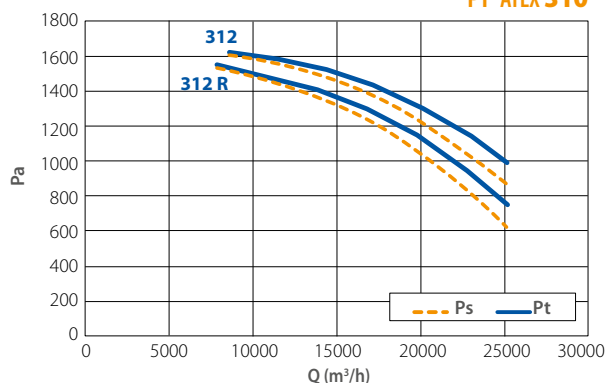
PF ATEX 310
