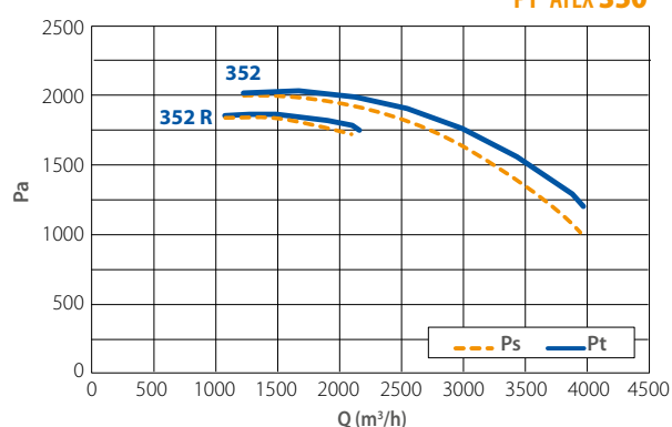
PF ATEX 350
