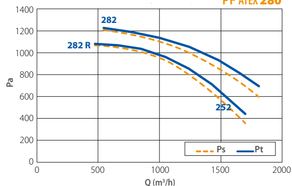
PF ATEX 280
