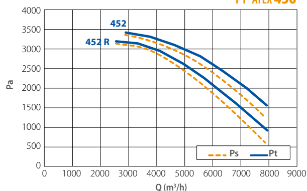
PF ATEX 450
